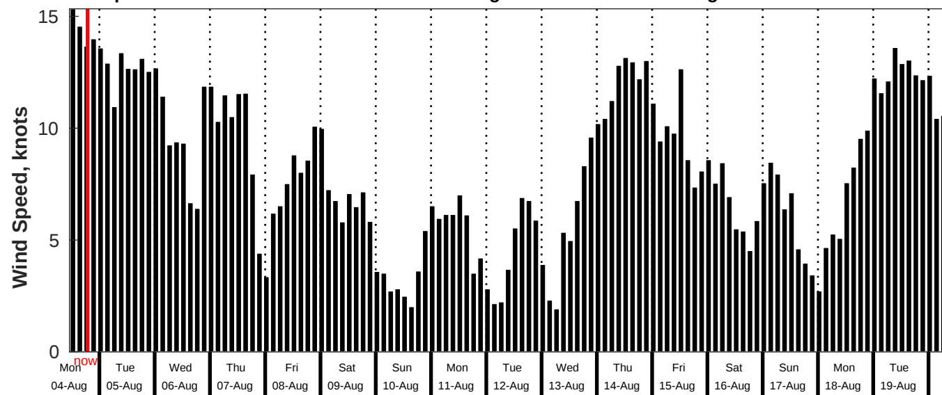
GFS Wind Speed Forecast for NDBC 52211 from 03-Aug-2025 11:00:00 to 19-Aug-2025 11:00:00
