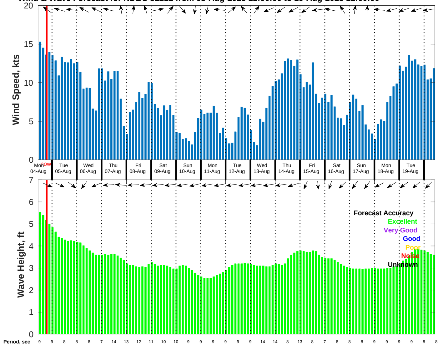
Wind & Wave Forecast for NDBC 52211 from 03-Aug-2025 11:00:00 to 19-Aug-2025 11:00:00
