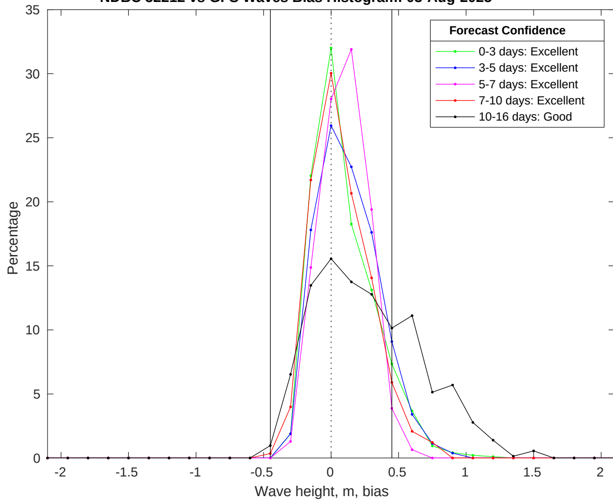
NDBC 52212 vs GFS Waves Bias Histogram: 03-Aug-2025
