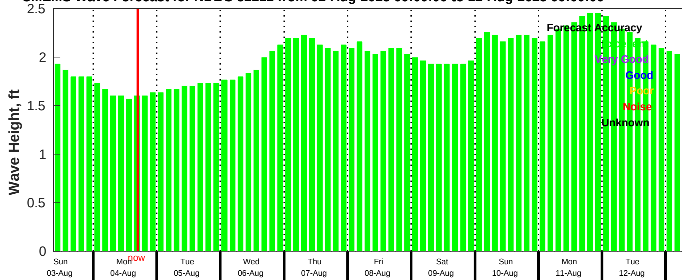
CMEMS Wave Forecast for NDBC 52212 from 02-Aug-2025 09:00:00 to 12-Aug-2025 09:00:00
