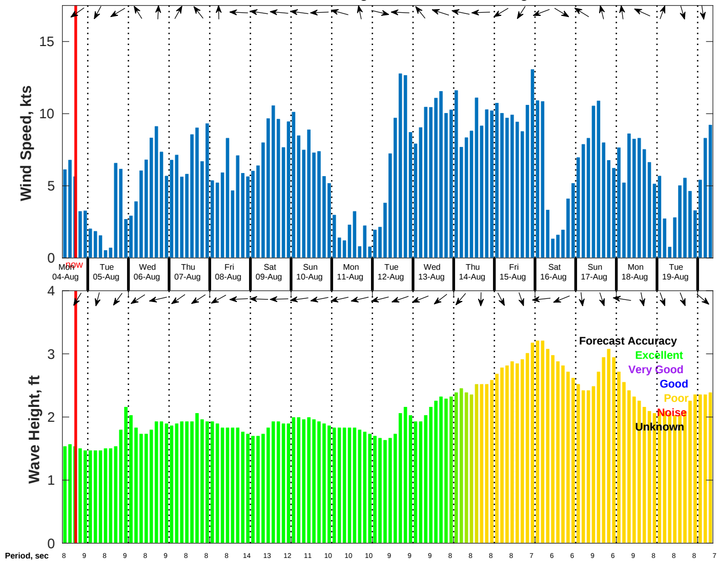
Wind & Wave Forecast for NDBC 52212 from 03-Aug-2025 09:00:00 to 19-Aug-2025 09:00:00
