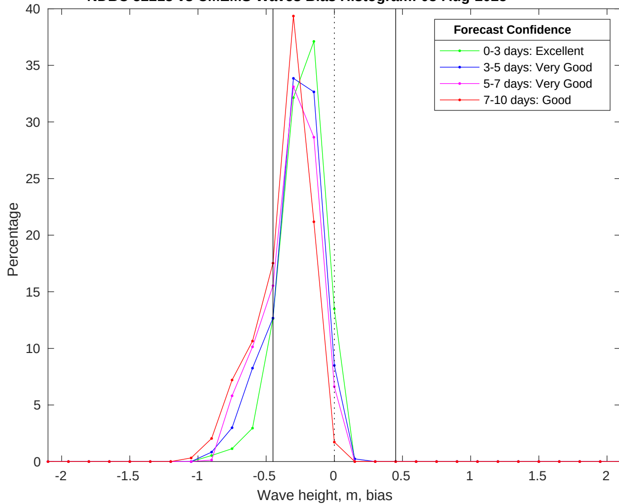
NDBC 52213 vs CMEMS Waves Bias Histogram: 03-Aug-2025
