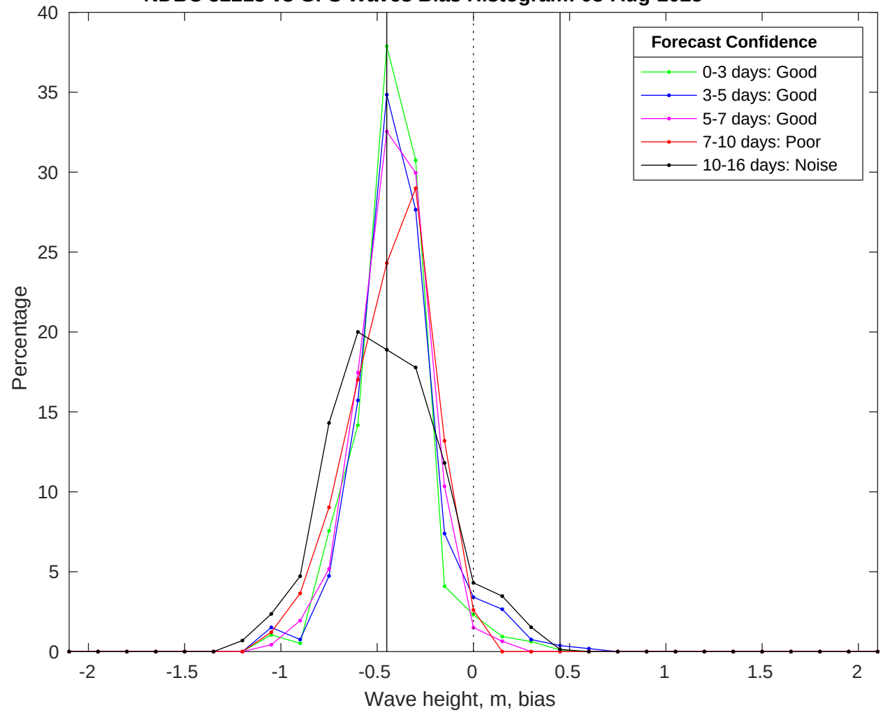
NDBC 52213 vs GFS Waves Bias Histogram: 03-Aug-2025
