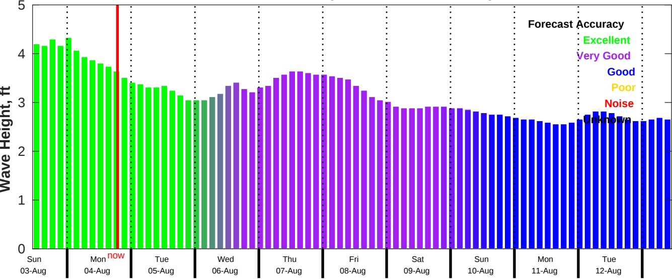
CMEMS Wave Forecast for NDBC 52213 from 02-Aug-2025 11:00:00 to 12-Aug-2025 11:00:00
