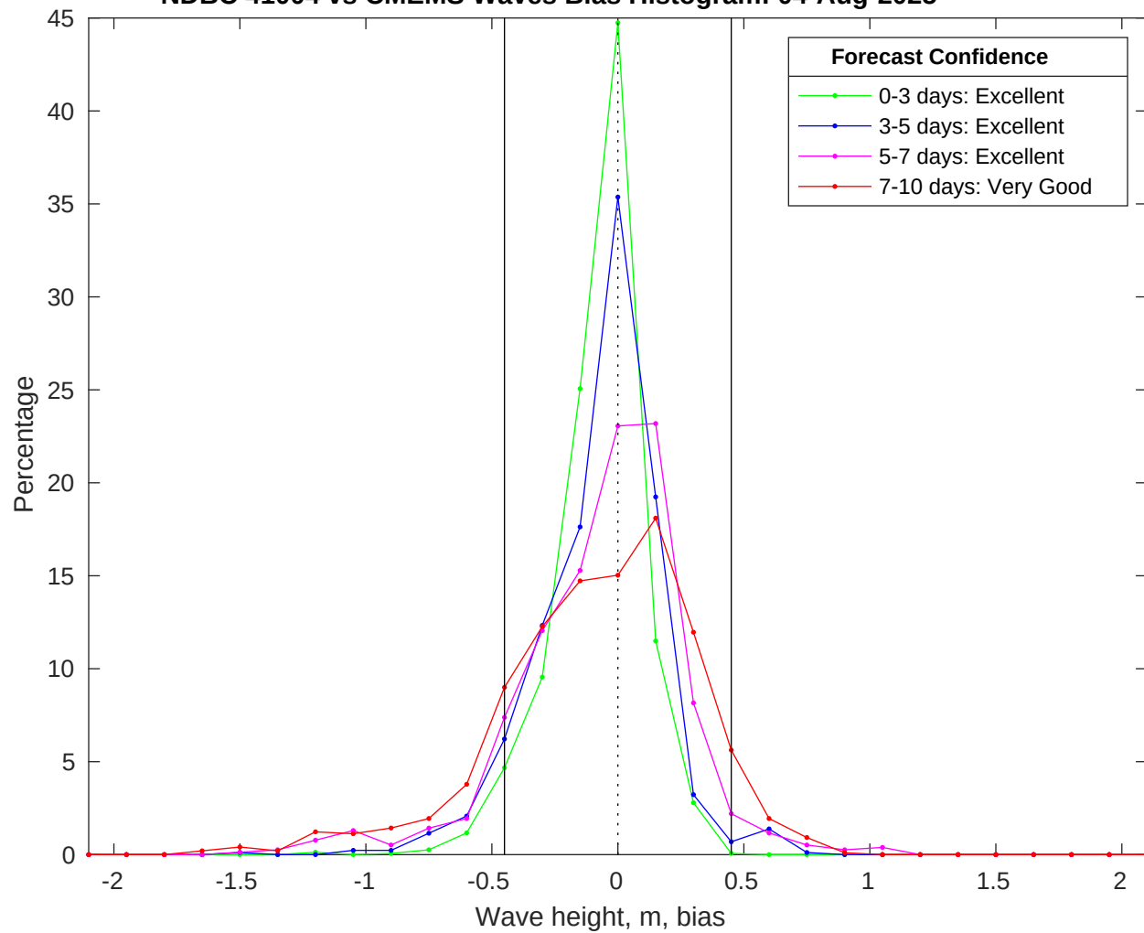
NDBC 41004 vs CMEMS Waves Bias Histogram: 04-Aug-2025
