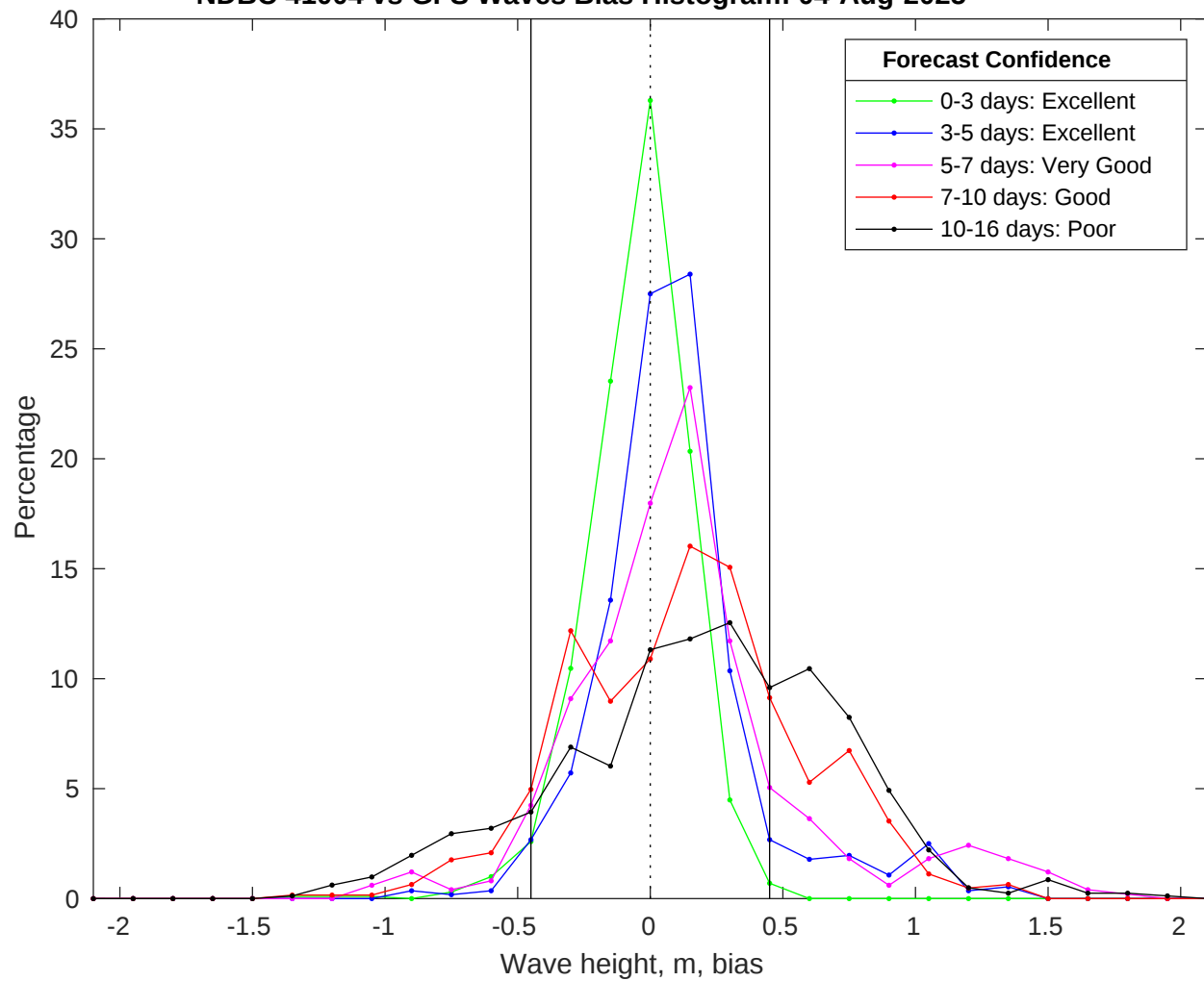
NDBC 41004 vs GFS Waves Bias Histogram: 04-Aug-2025
