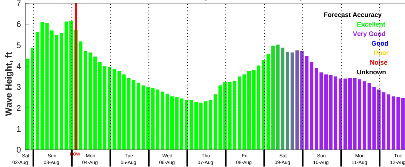
CMEMS Wave Forecast for NDBC 41004 from 02-Aug-2025 19:00:00 to 12-Aug-2025 19:00:00
