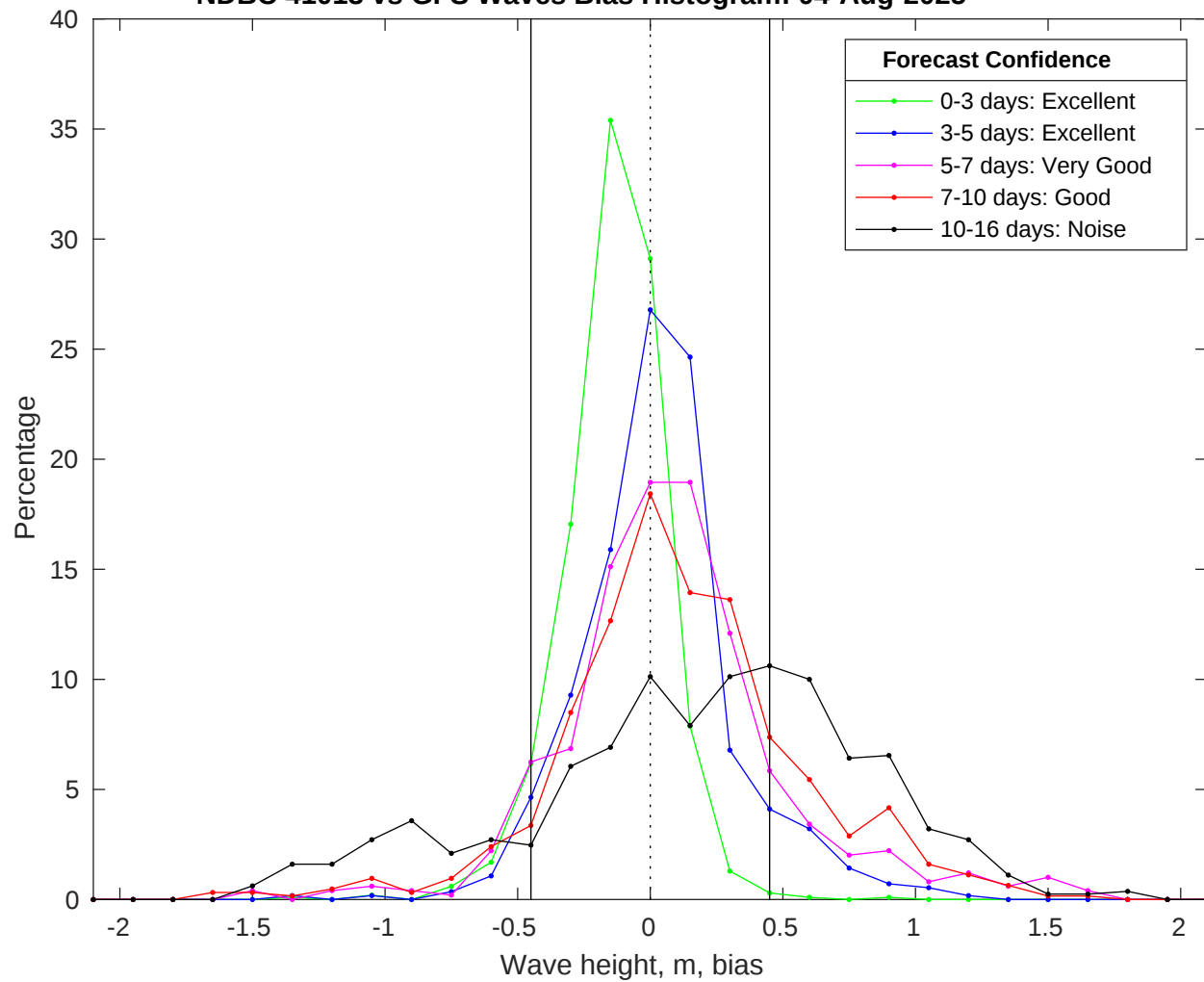
NDBC 41013 vs GFS Waves Bias Histogram: 04-Aug-2025
