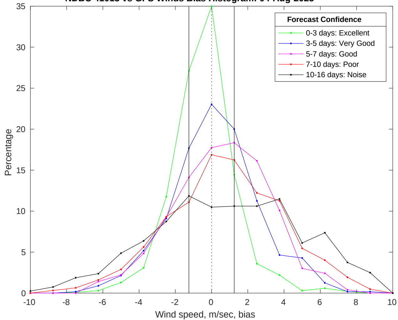
NDBC 41013 vs GFS Winds Bias Histogram: 04-Aug-2025
