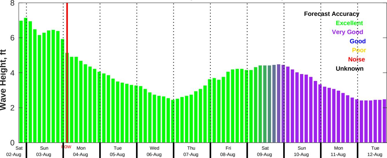
CMEMS Wave Forecast for NDBC 41013 from 02-Aug-2025 19:00:00 to 12-Aug-2025 19:00:00
