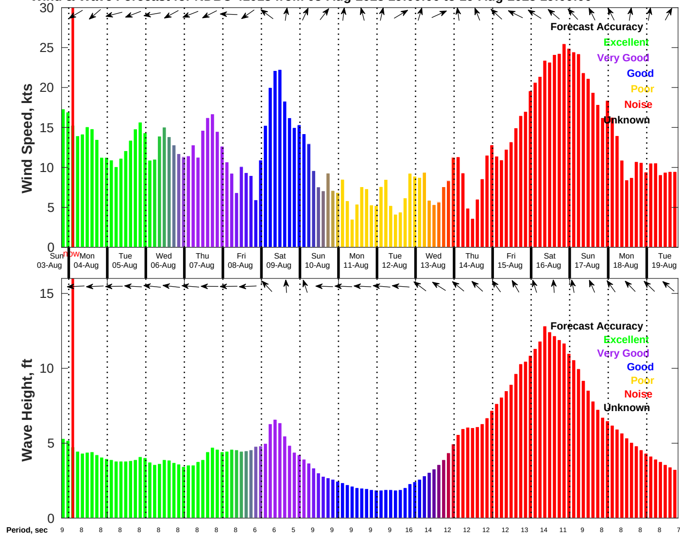
Wind & Wave Forecast for NDBC 41013 from 03-Aug-2025 19:00:00 to 19-Aug-2025 19:00:00
