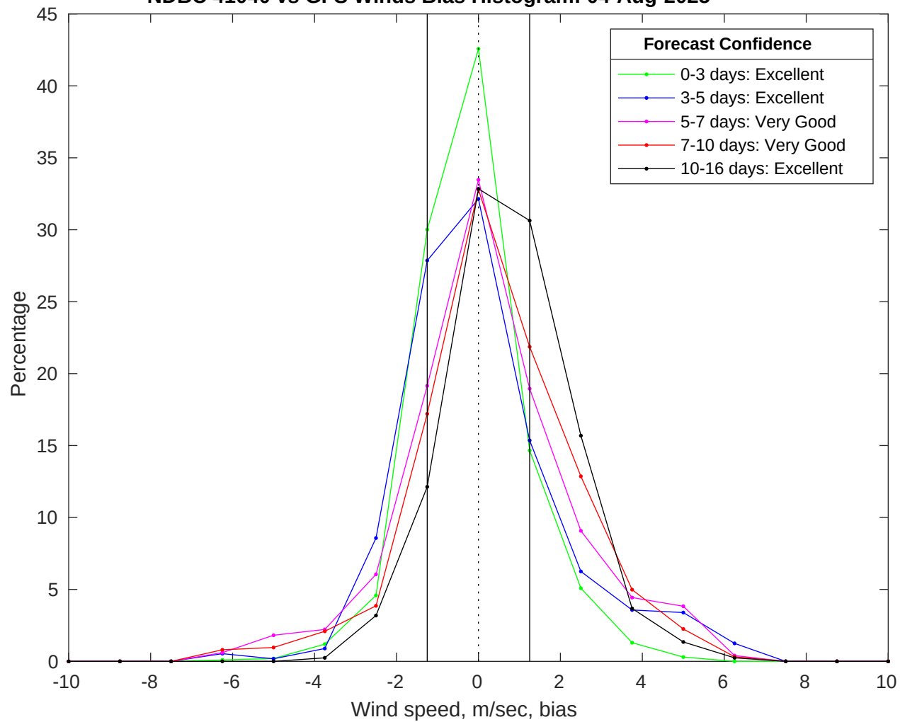
NDBC 41040 vs GFS Winds Bias Histogram: 04-Aug-2025
