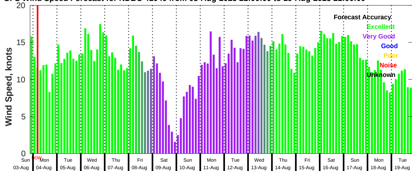
GFS Wind Speed Forecast for NDBC 41040 from 03-Aug-2025 21:00:00 to 19-Aug-2025 21:00:00
