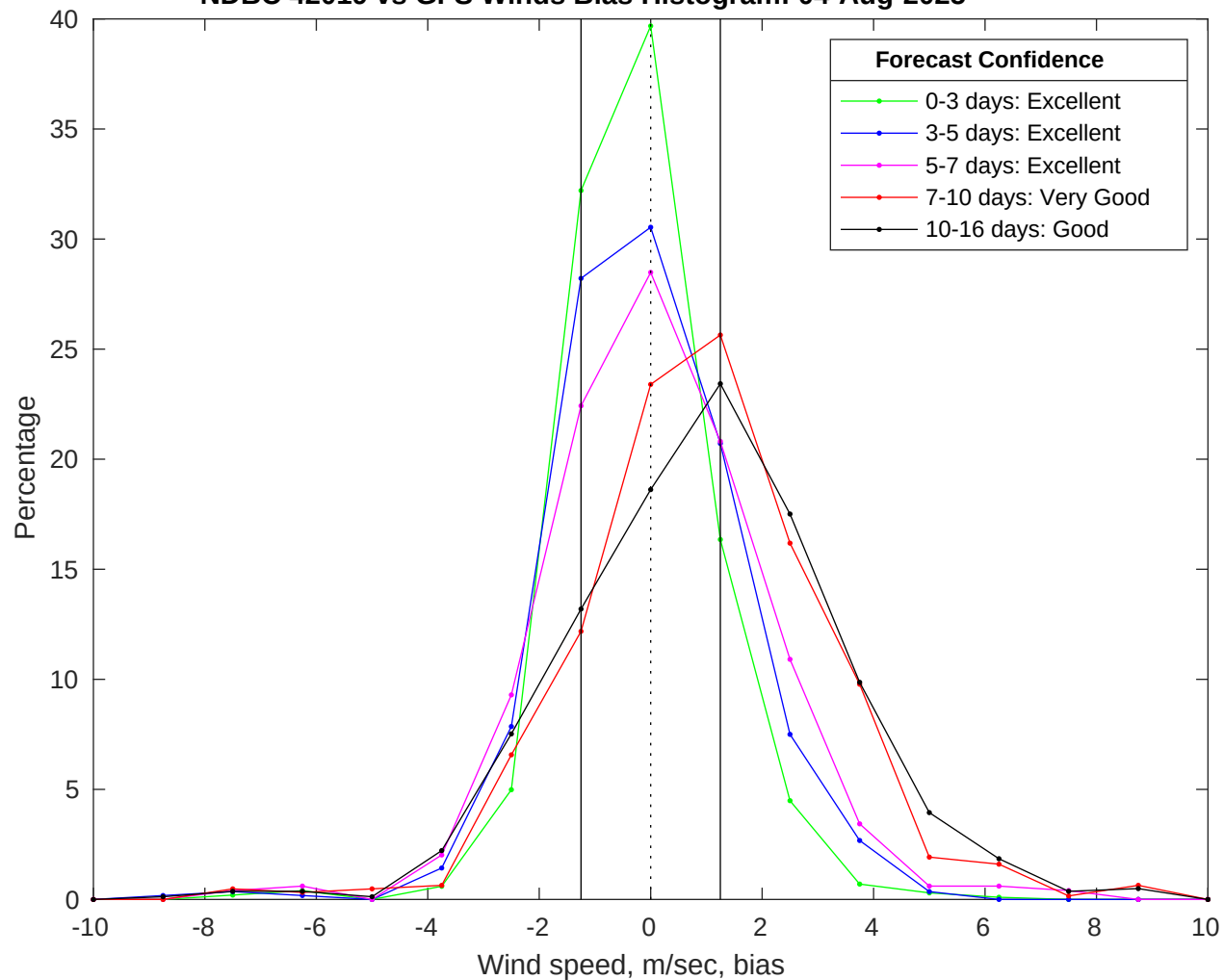
NDBC 42019 vs GFS Winds Bias Histogram: 04-Aug-2025
