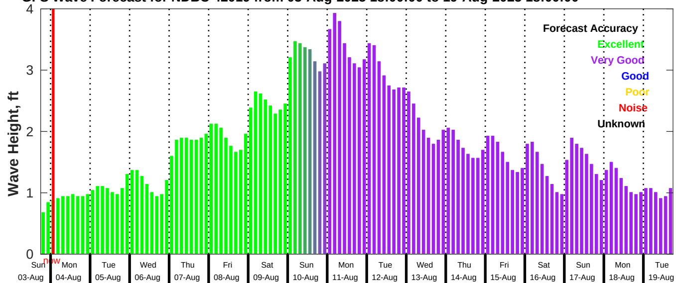
GFS Wave Forecast for NDBC 42019 from 03-Aug-2025 18:00:00 to 19-Aug-2025 18:00:00
