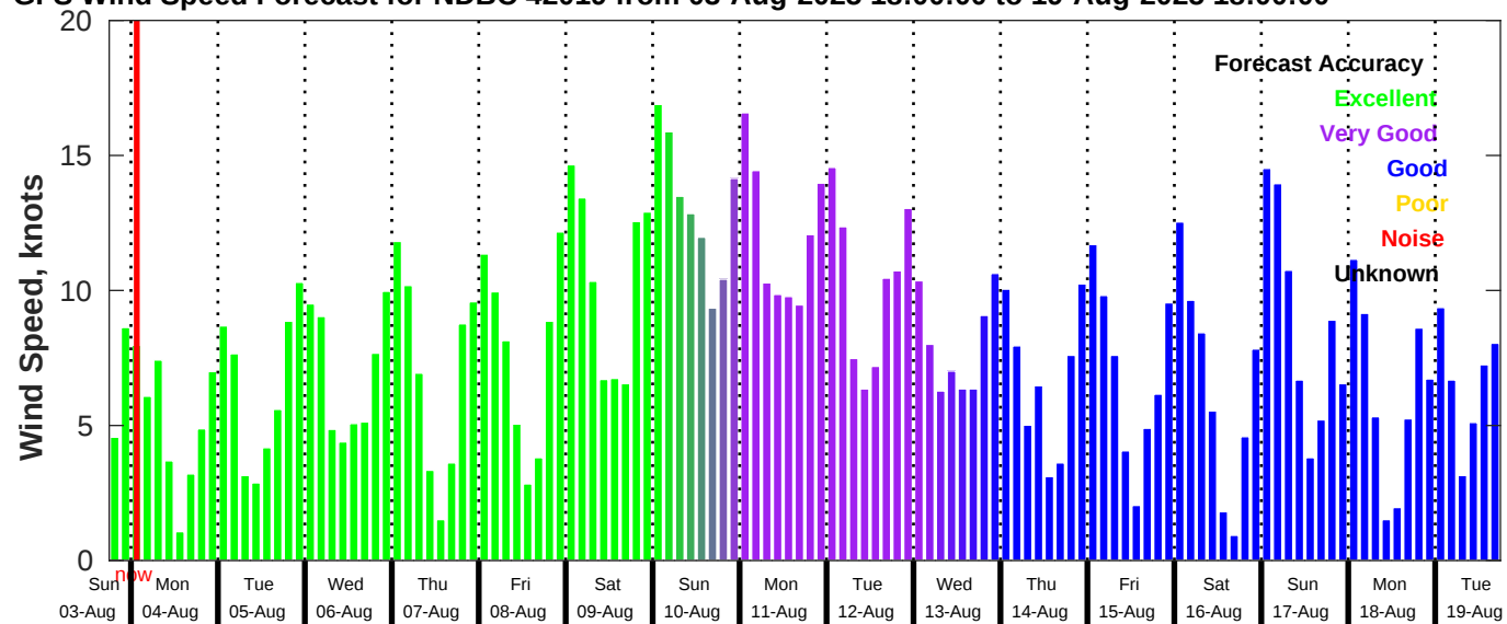
GFS Wind Speed Forecast for NDBC 42019 from 03-Aug-2025 18:00:00 to 19-Aug-2025 18:00:00
