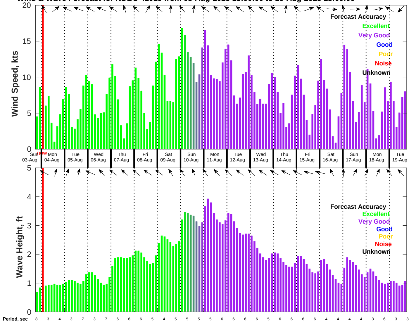
Wind & Wave Forecast for NDBC 42019 from 03-Aug-2025 18:00:00 to 19-Aug-2025 18:00:00
