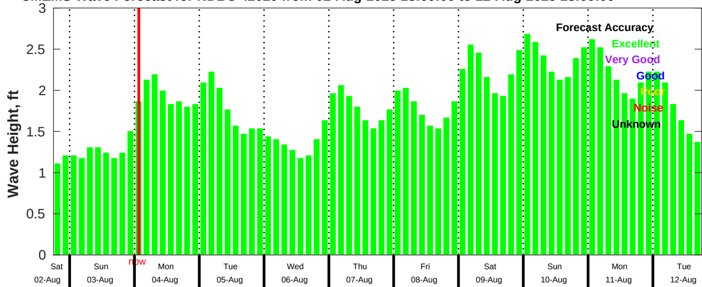
CMEMS Wave Forecast for NDBC 42020 from 02-Aug-2025 18:00:00 to 12-Aug-2025 18:00:00
