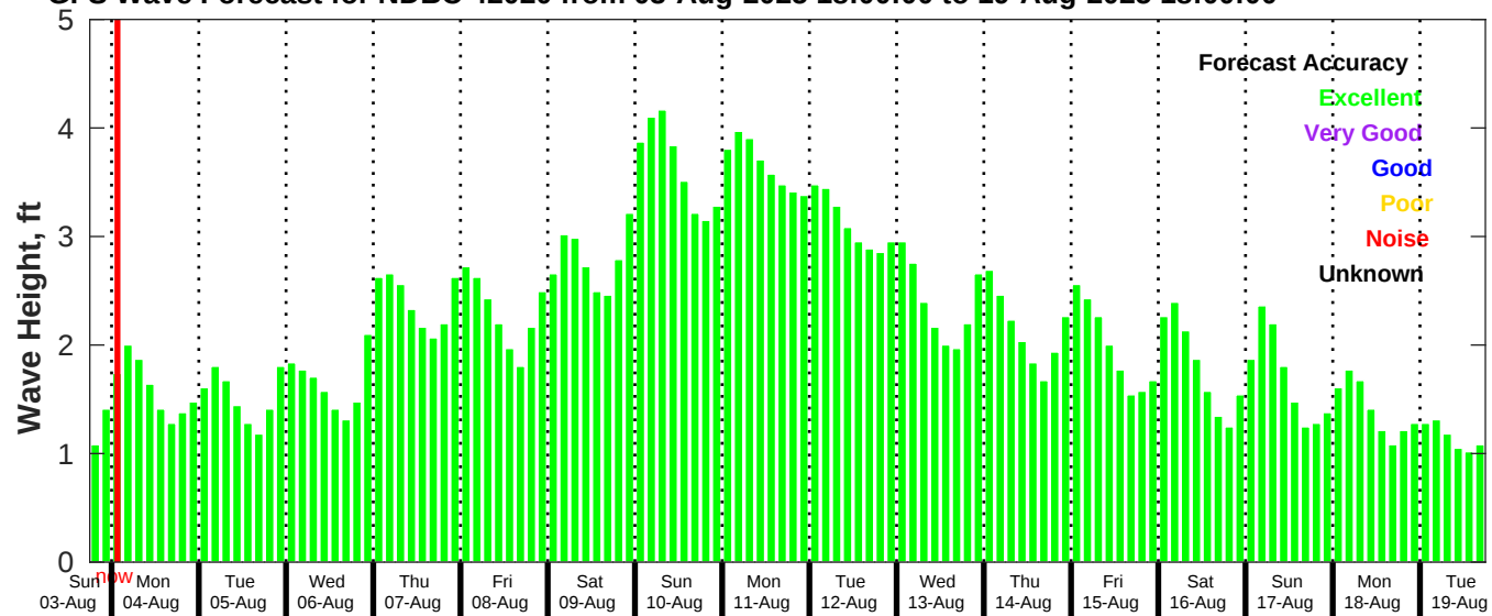
GFS Wave Forecast for NDBC 42020 from 03-Aug-2025 18:00:00 to 19-Aug-2025 18:00:00
