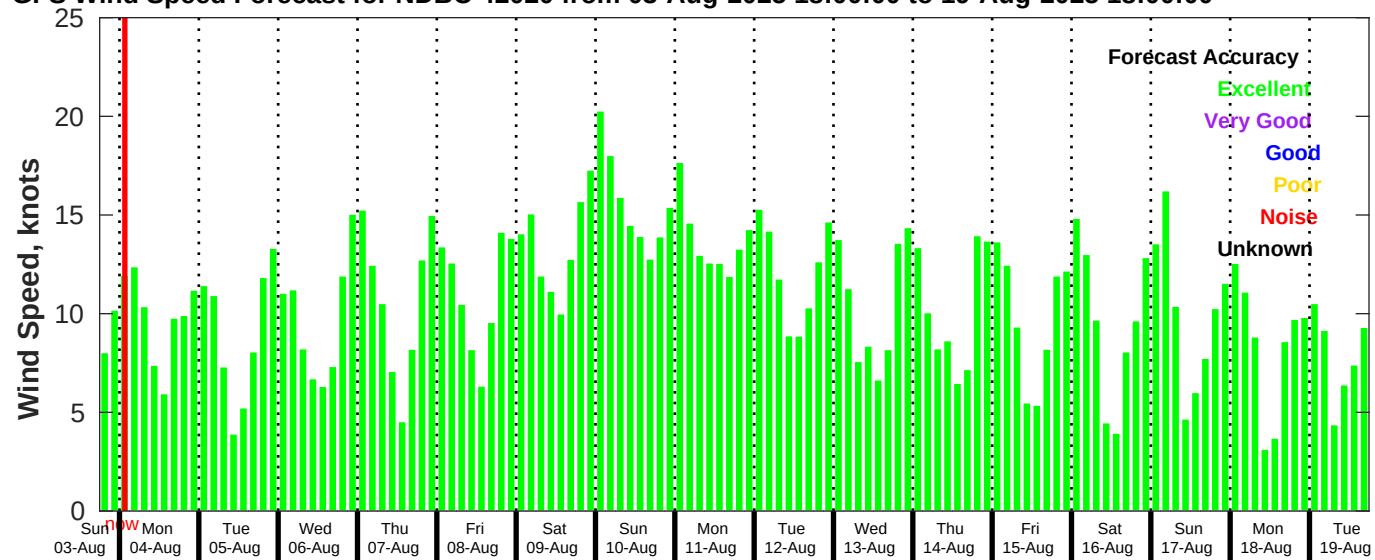
GFS Wind Speed Forecast for NDBC 42020 from 03-Aug-2025 18:00:00 to 19-Aug-2025 18:00:00
