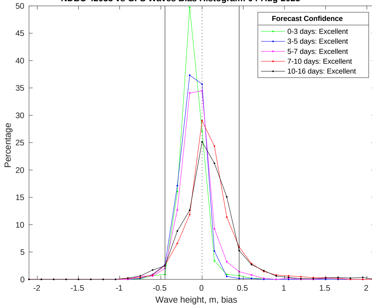
NDBC 42035 vs GFS Waves Bias Histogram: 04-Aug-2025
