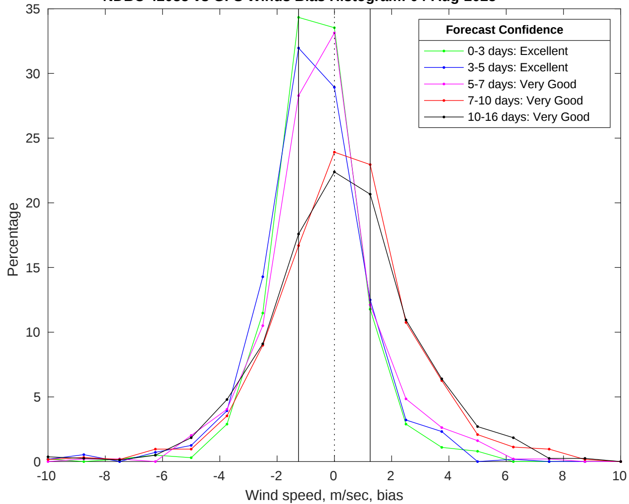
NDBC 42035 vs GFS Winds Bias Histogram: 04-Aug-2025
