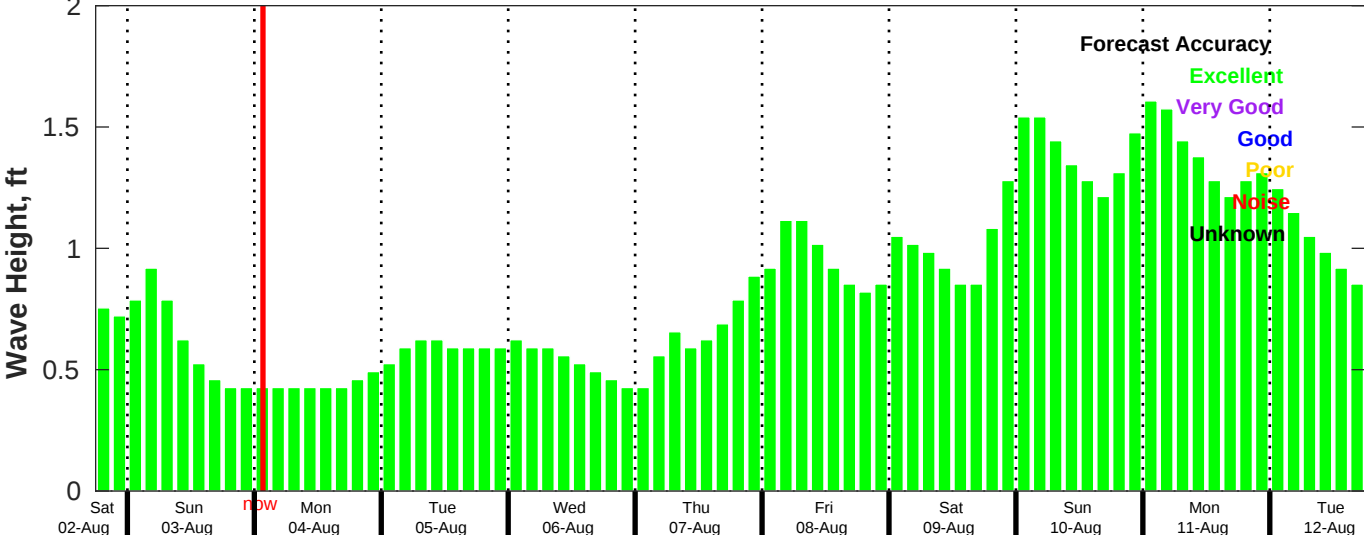
CMEMS Wave Forecast for NDBC 42035 from 02-Aug-2025 18:00:00 to 12-Aug-2025 18:00:00
