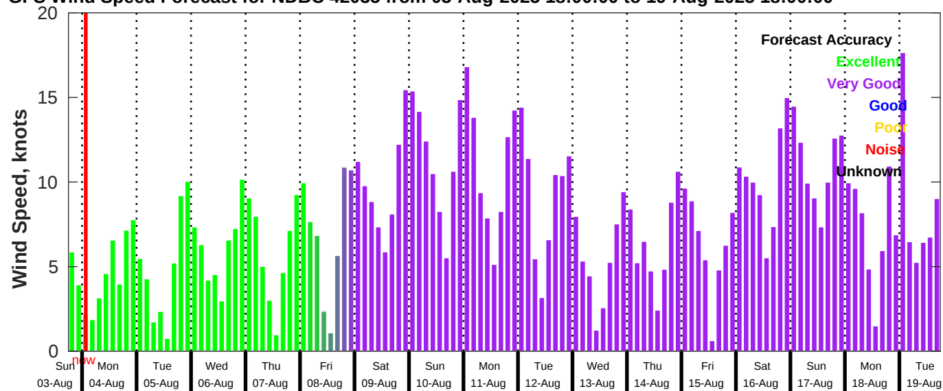
GFS Wind Speed Forecast for NDBC 42035 from 03-Aug-2025 18:00:00 to 19-Aug-2025 18:00:00
