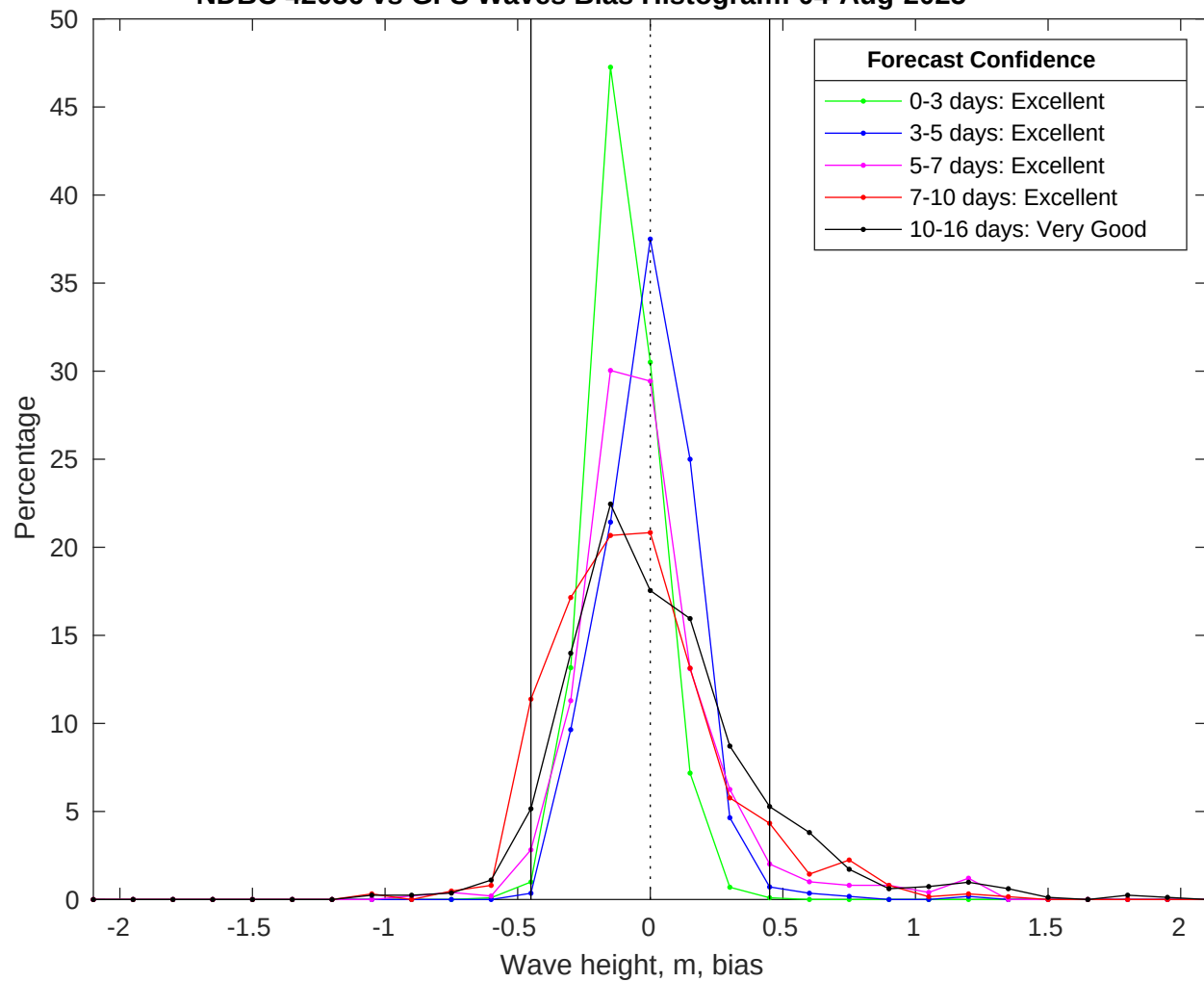
NDBC 42036 vs GFS Waves Bias Histogram: 04-Aug-2025
