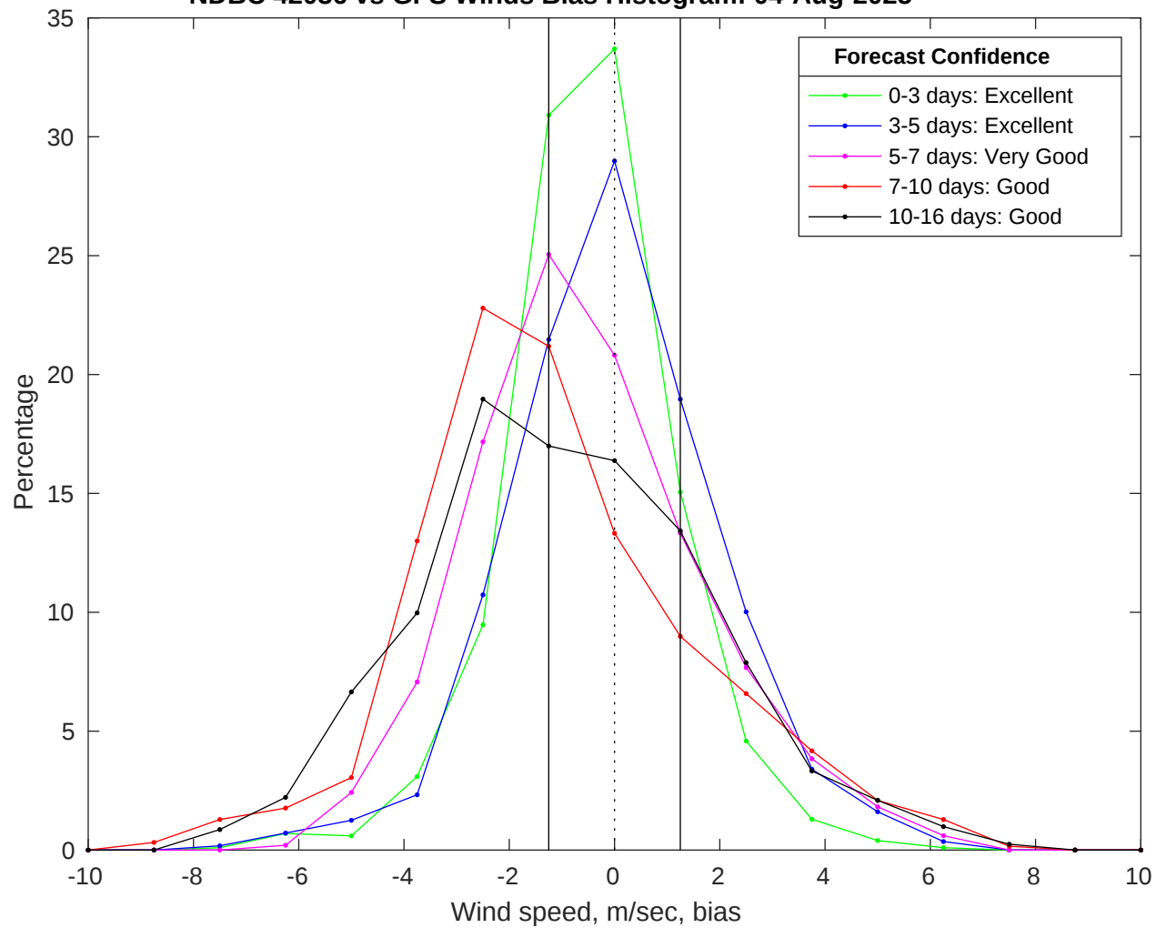
NDBC 42036 vs GFS Winds Bias Histogram: 04-Aug-2025
