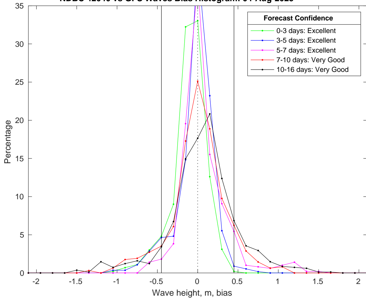
NDBC 42040 vs GFS Waves Bias Histogram: 04-Aug-2025
