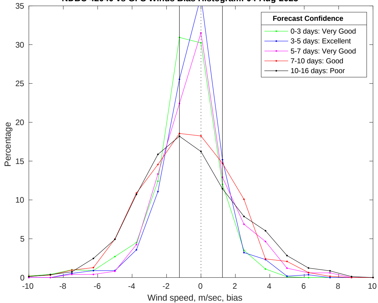
NDBC 42040 vs GFS Winds Bias Histogram: 04-Aug-2025
