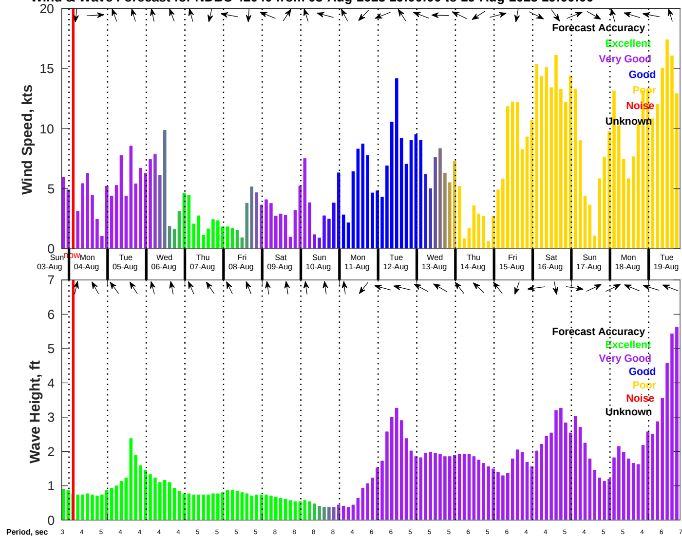
Wind & Wave Forecast for NDBC 42040 from 03-Aug-2025 19:00:00 to 19-Aug-2025 19:00:00
