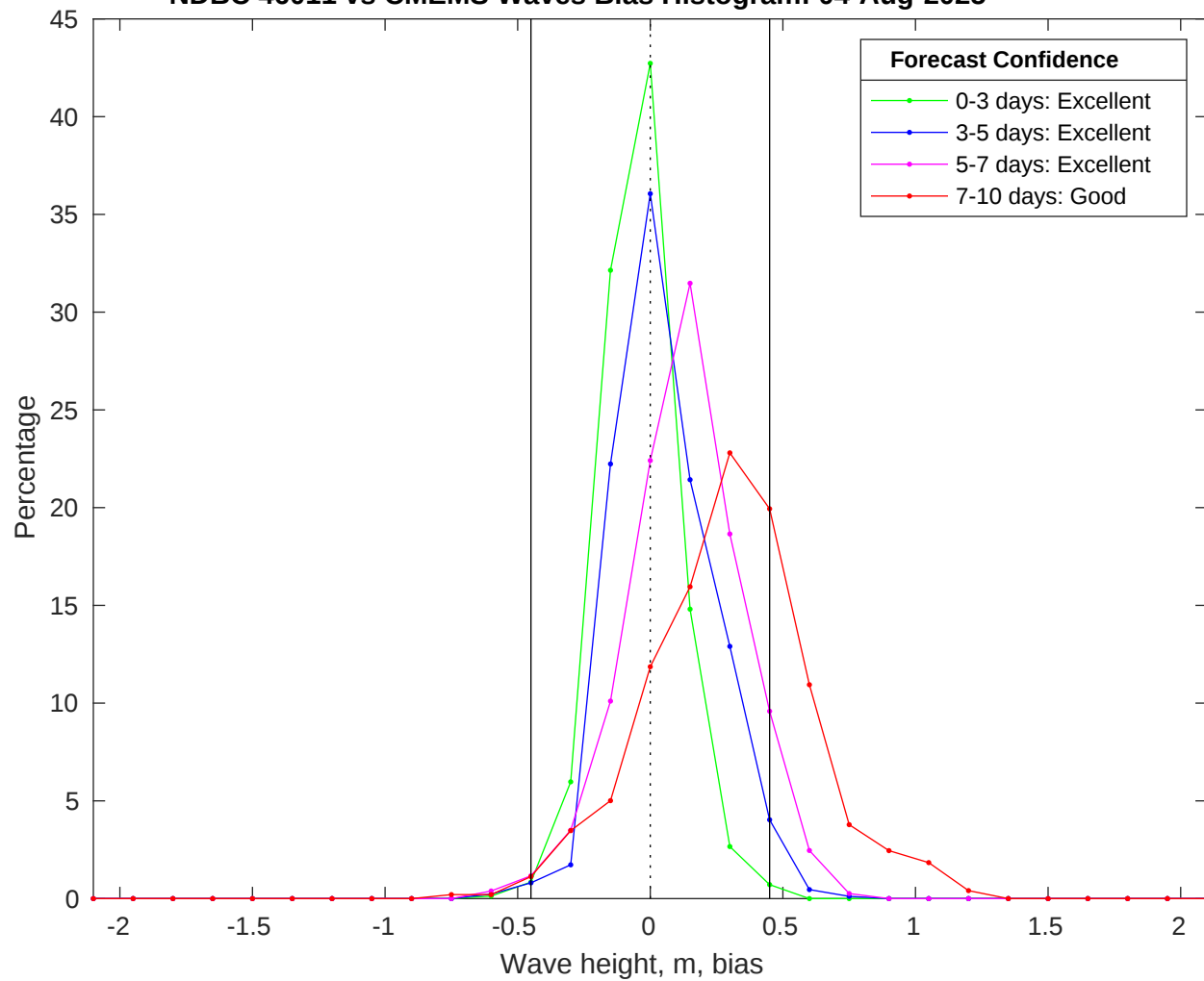
NDBC 46011 vs CMEMS Waves Bias Histogram: 04-Aug-2025
