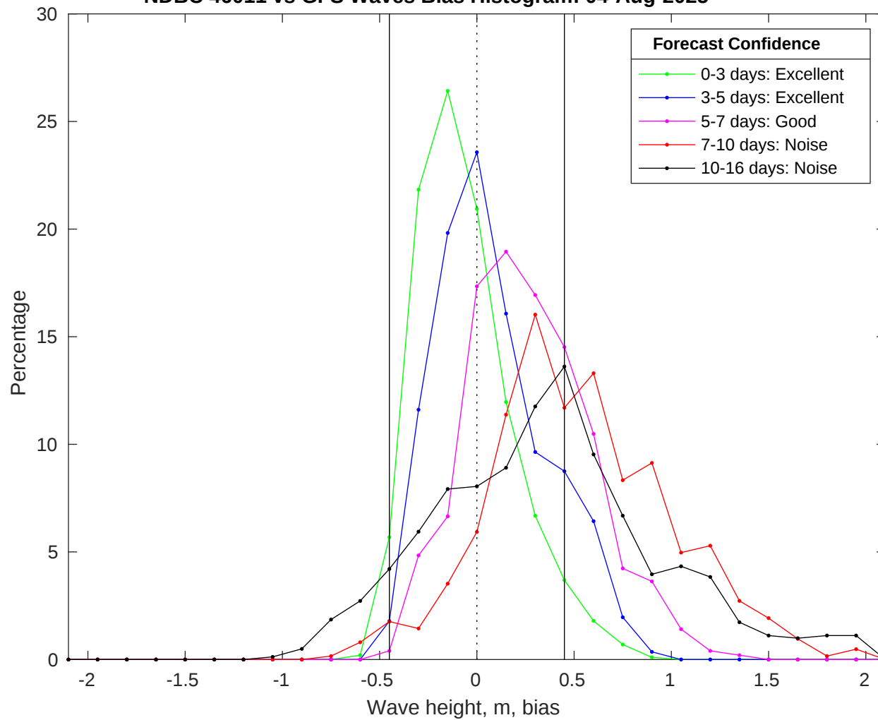
NDBC 46011 vs GFS Waves Bias Histogram: 04-Aug-2025
