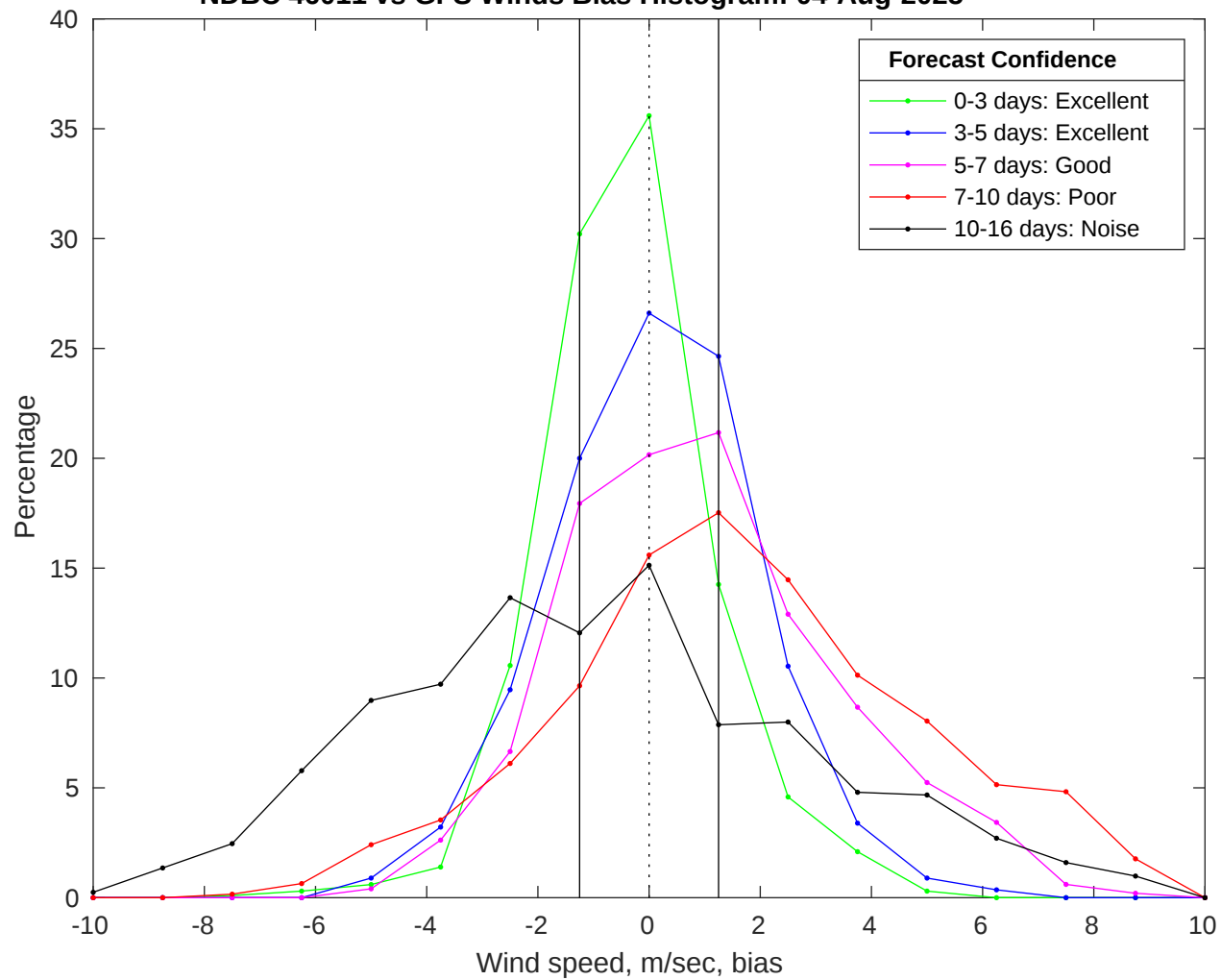
NDBC 46011 vs GFS Winds Bias Histogram: 04-Aug-2025
