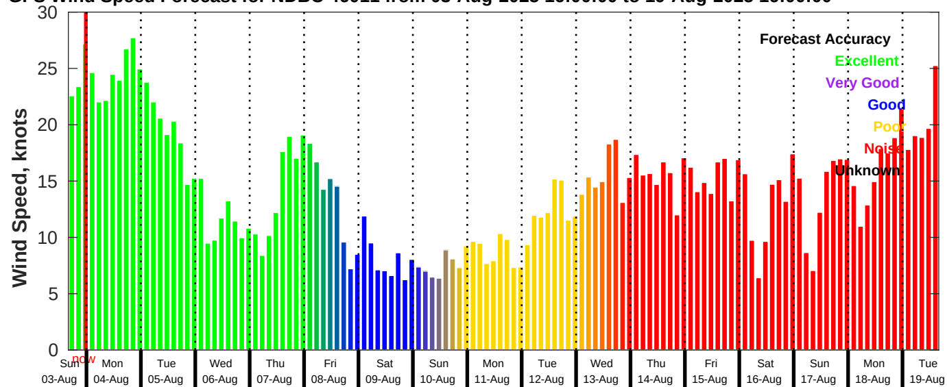
GFS Wind Speed Forecast for NDBC 46011 from 03-Aug-2025 16:00:00 to 19-Aug-2025 16:00:00
