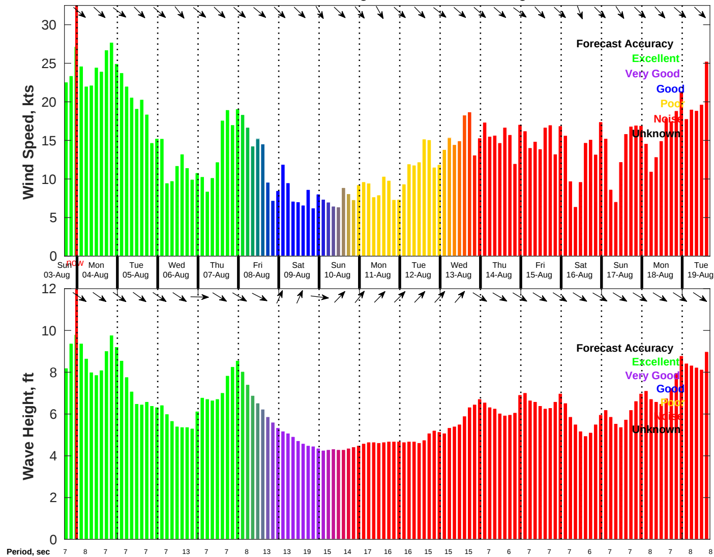
Wind & Wave Forecast for NDBC 46011 from 03-Aug-2025 16:00:00 to 19-Aug-2025 16:00:00
