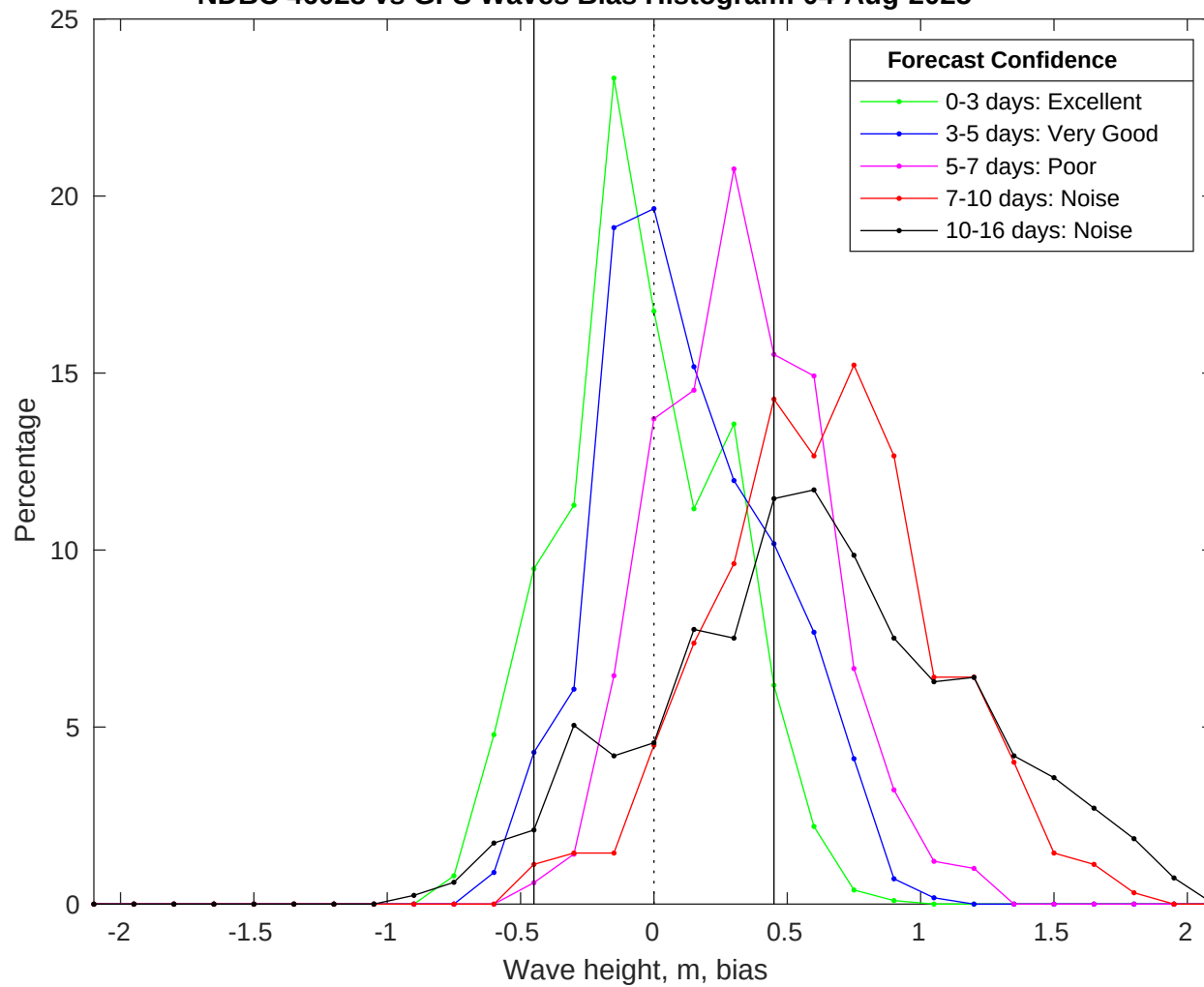
NDBC 46028 vs GFS Waves Bias Histogram: 04-Aug-2025
