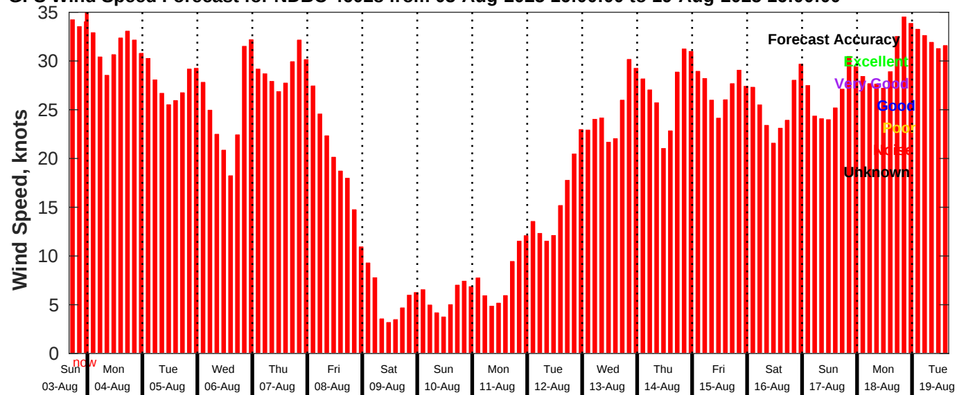
GFS Wind Speed Forecast for NDBC 46028 from 03-Aug-2025 16:00:00 to 19-Aug-2025 16:00:00
