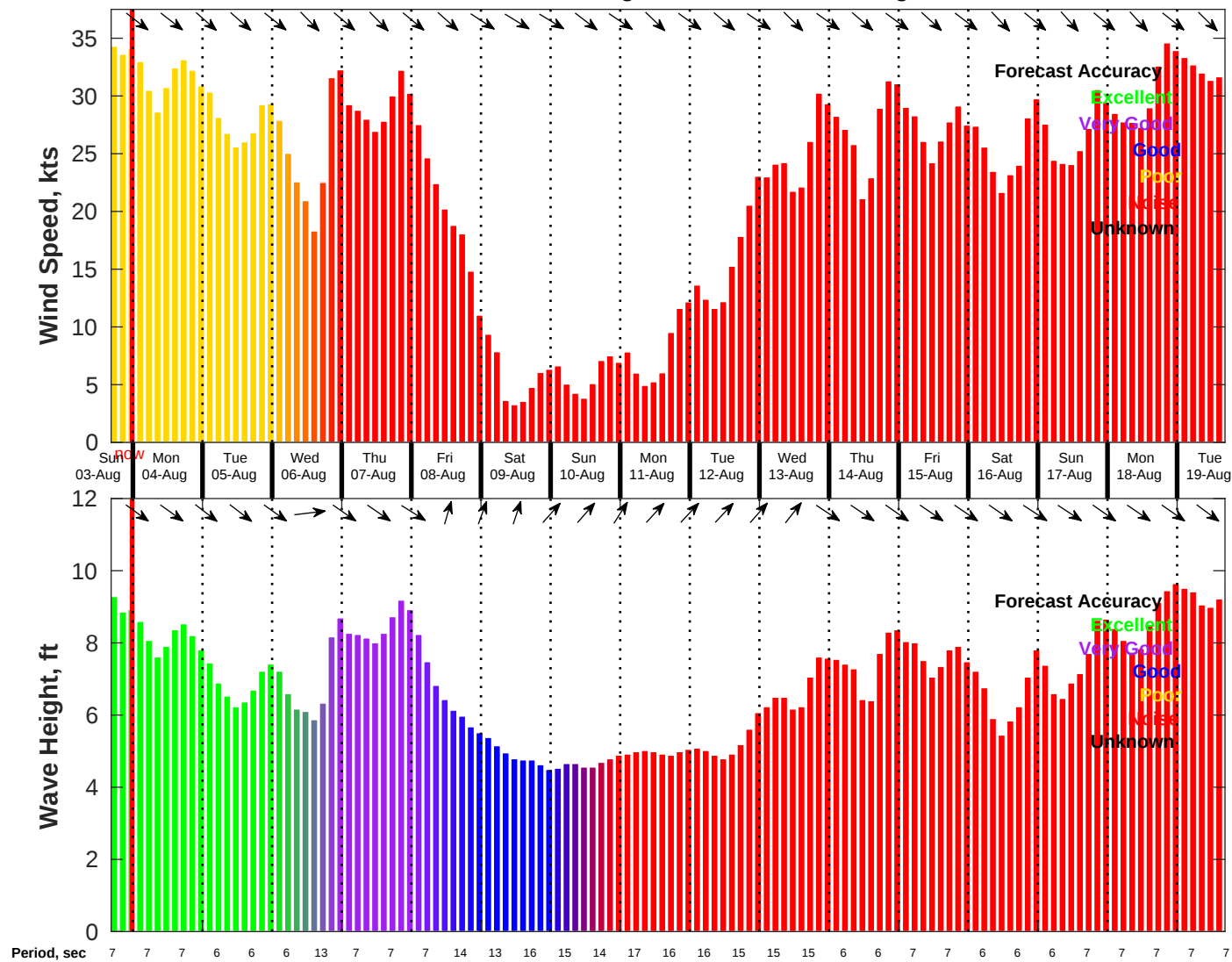
Wind & Wave Forecast for NDBC 46028 from 03-Aug-2025 16:00:00 to 19-Aug-2025 16:00:00
