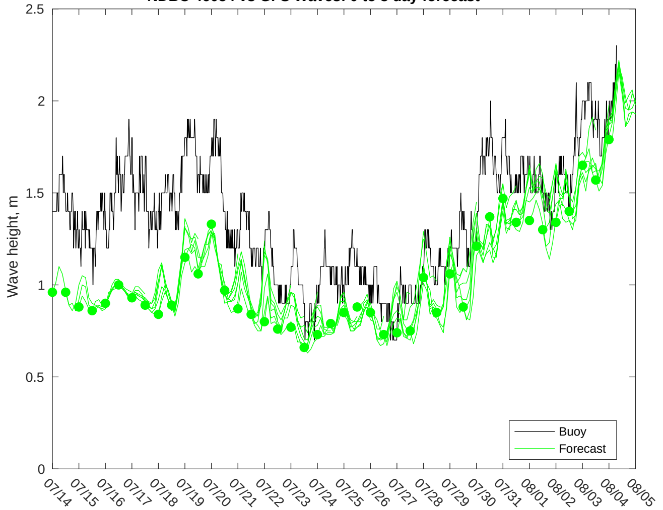
NDBC 46054 vs GFS Waves: 0 to 3 day forecast
