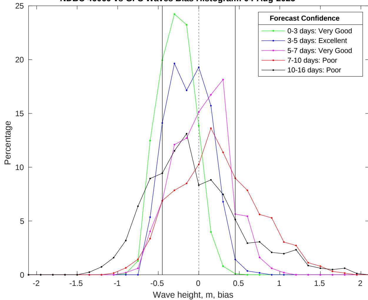
NDBC 46069 vs GFS Waves Bias Histogram: 04-Aug-2025
