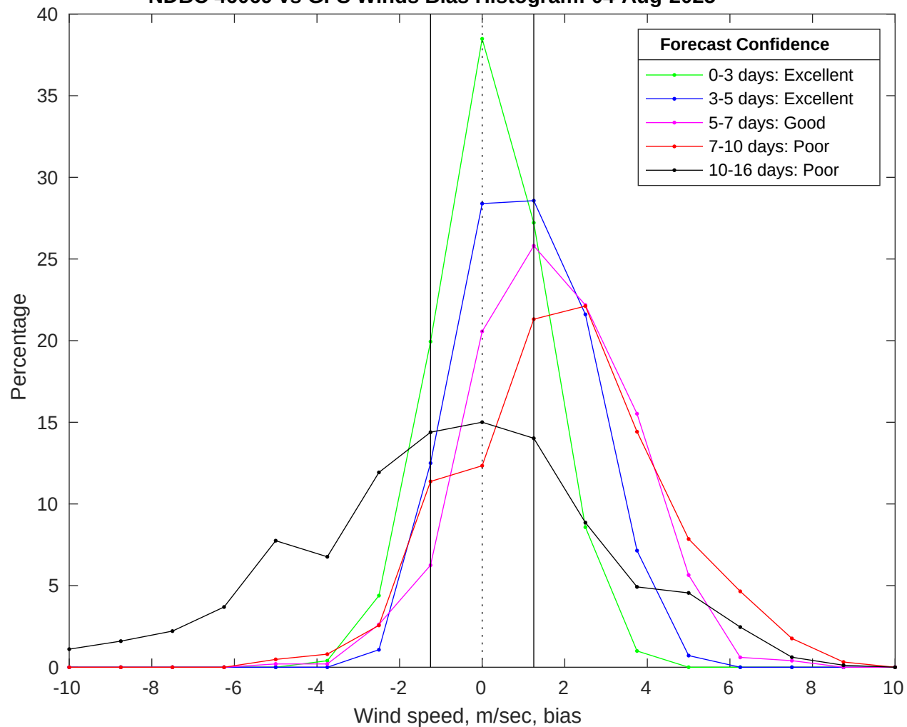
NDBC 46069 vs GFS Winds Bias Histogram: 04-Aug-2025
