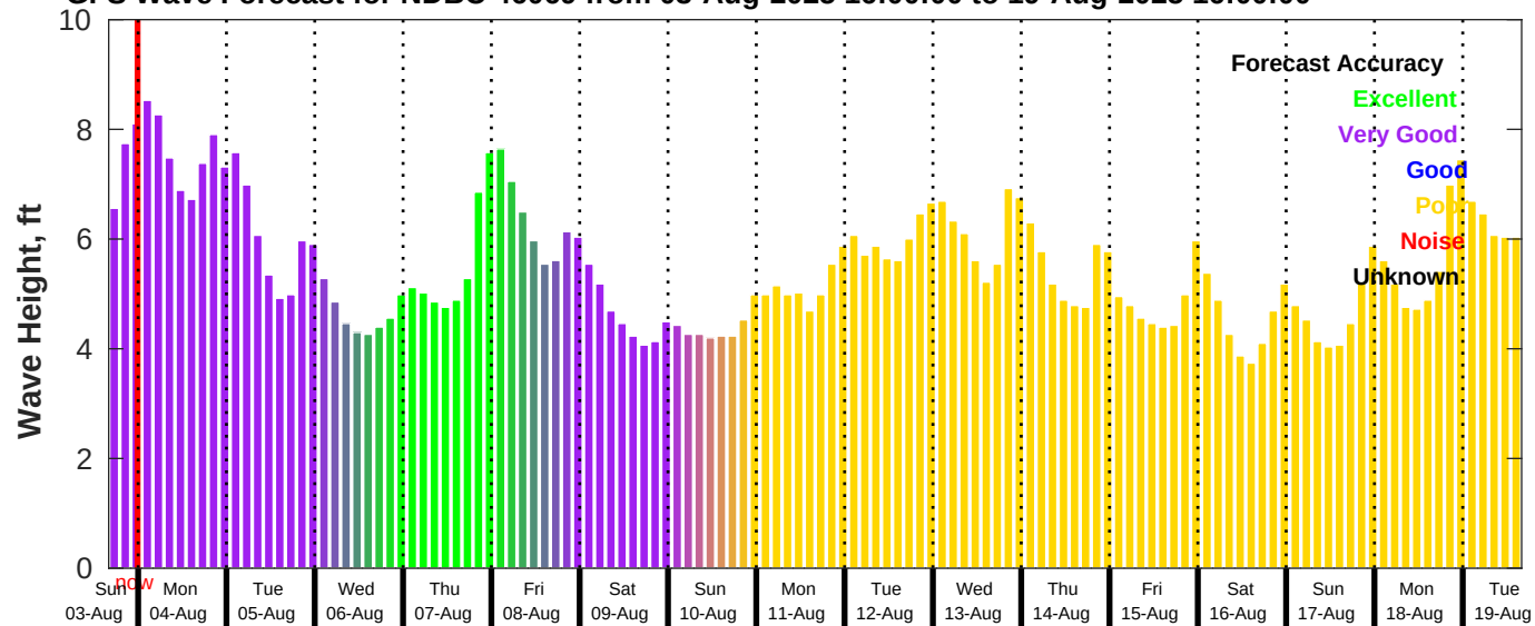
GFS Wave Forecast for NDBC 46069 from 03-Aug-2025 16:00:00 to 19-Aug-2025 16:00:00
