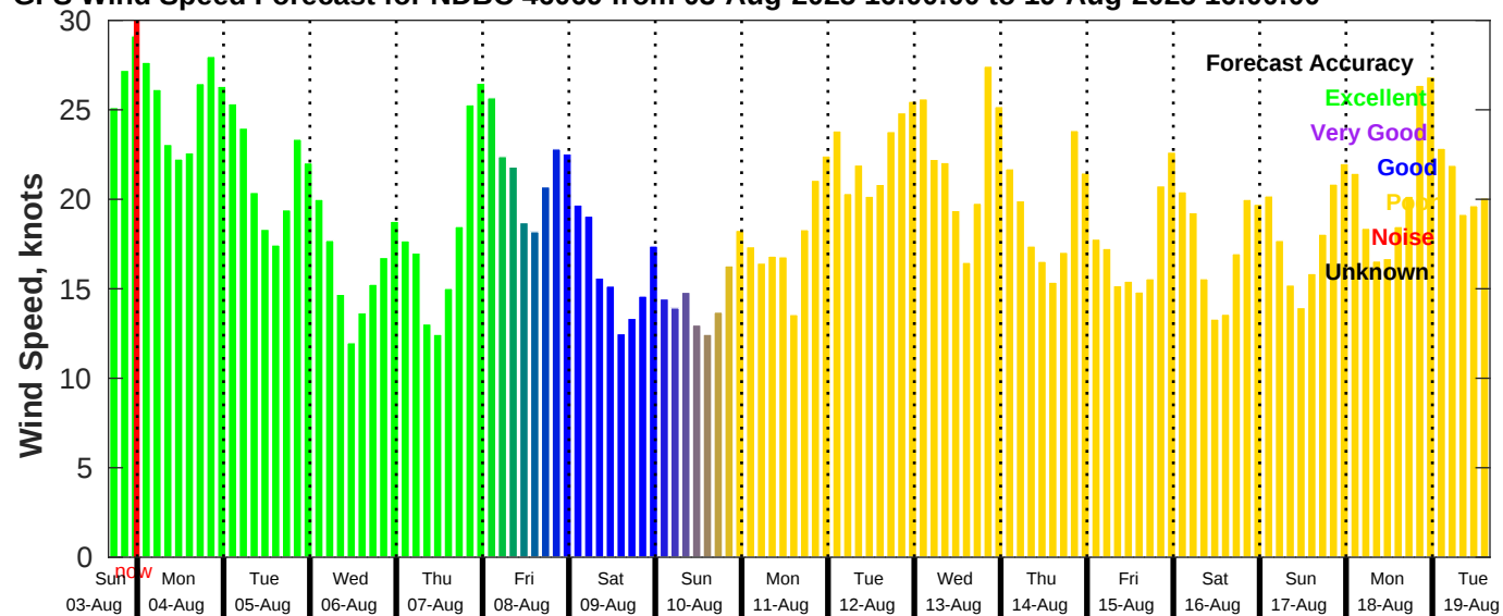
GFS Wind Speed Forecast for NDBC 46069 from 03-Aug-2025 16:00:00 to 19-Aug-2025 16:00:00
