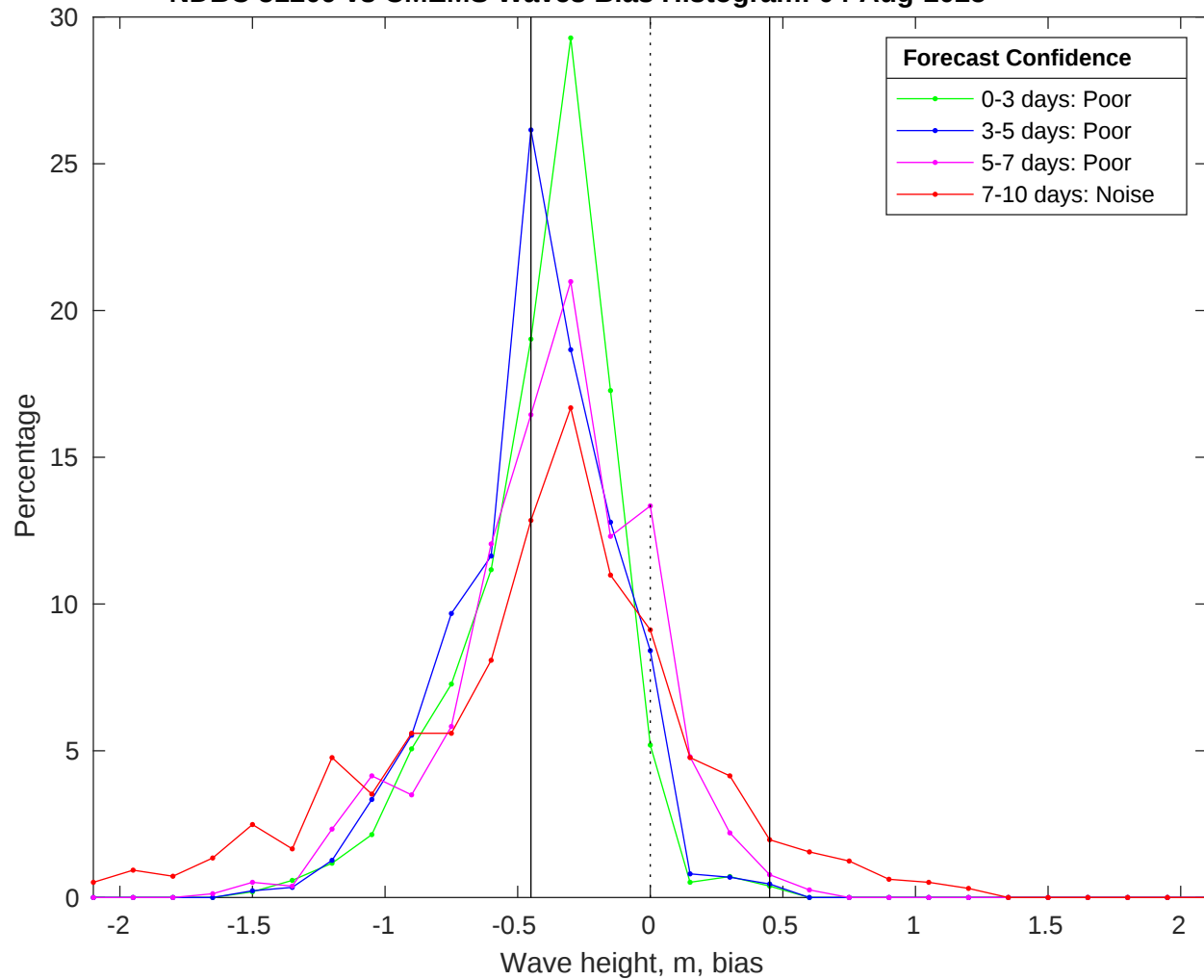
NDBC 51209 vs CMEMS Waves Bias Histogram: 04-Aug-2025
