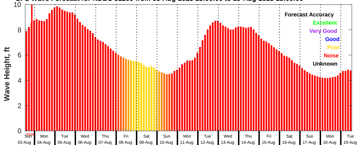
GFS Wave Forecast for NDBC 51209 from 03-Aug-2025 13:00:00 to 19-Aug-2025 13:00:00
