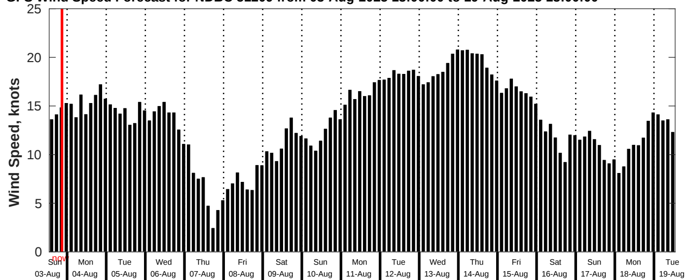
GFS Wind Speed Forecast for NDBC 51209 from 03-Aug-2025 13:00:00 to 19-Aug-2025 13:00:00
