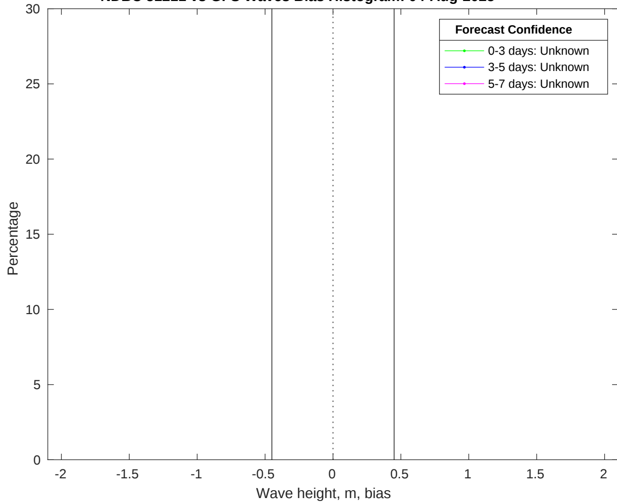
NDBC 51211 vs GFS Waves Bias Histogram: 04-Aug-2025
